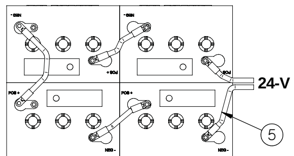
(4) 6-V BATTERY WIRING DIAGRAM
